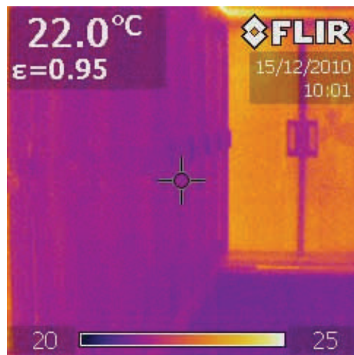
Enclosed cold aisle temperature analysis
