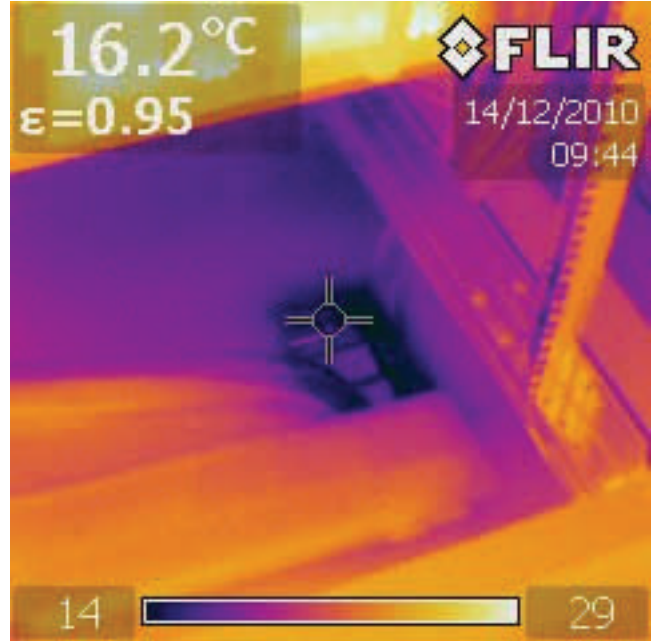
Cold air escaping under a rack where a brush grommet should have been placed
