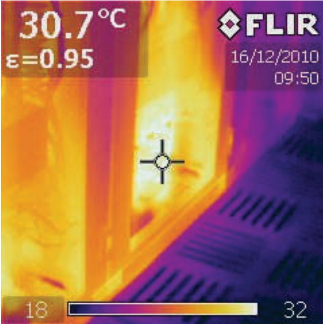
IT equipment the 'wrong way round' i.e. blowing hot exhaust air back into the cold aisle
